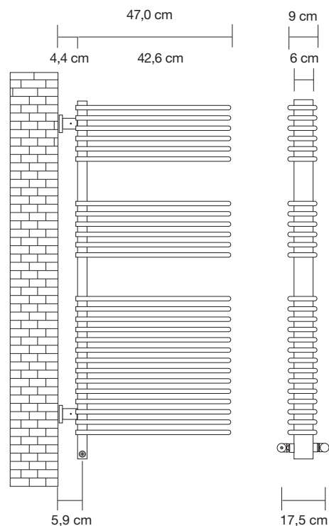
Inter-axis between connectors with sizes based on Tubes valves
