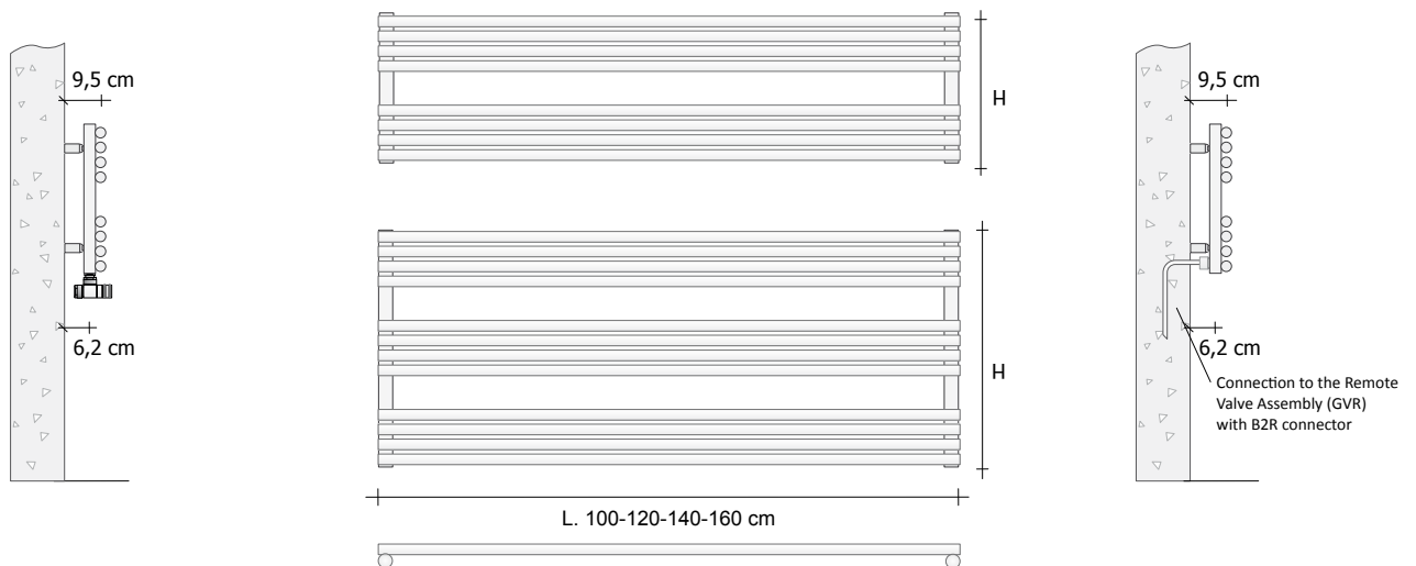
STANDARD HYDRAULIC VERSION (Connectors OB1)
