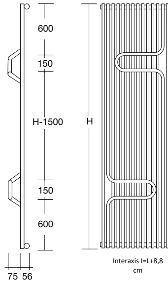
STANDARD HYDRAULIC AK2 - VERSION WITH DOUBLE HANDLE (Connectors OC1)
