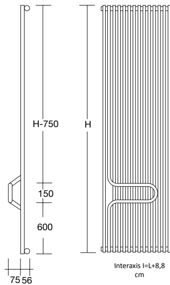
STANDARD HYDRAULIC AK - VERSION (Connectors OC1)
